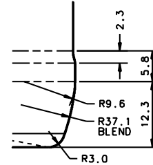
INSWEEP AND HEEL DETAIL SCALE 2:1
