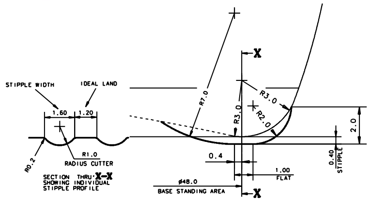
STIPPLE DETAIL SCALE 10:1
