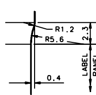
LABEL PANEL DETAIL SCALE 5:1
