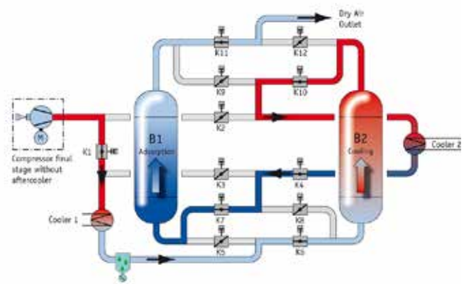
Cooling phase
