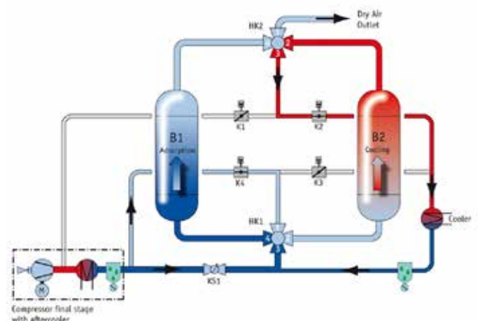
Cooling phase
