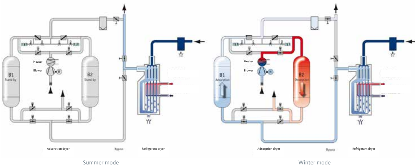
Summer mode
