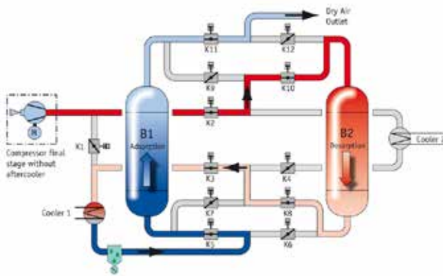
Desorption phase
