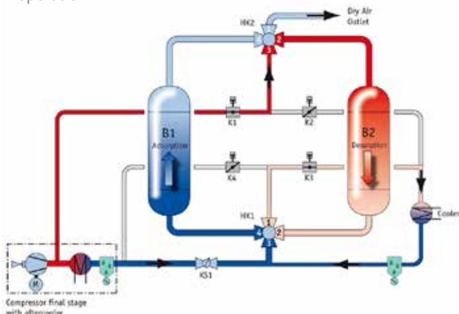
Desorption phase
