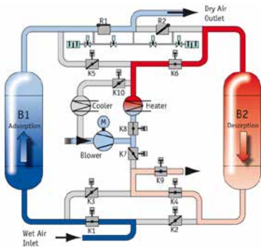
Desorption phase
