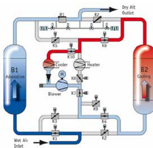
Cooling phase
