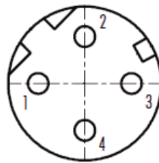
4 pole female socket with wires (front view)
