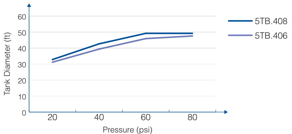
Overview of the tank diameter, depending upon the pressure of series 5TB
