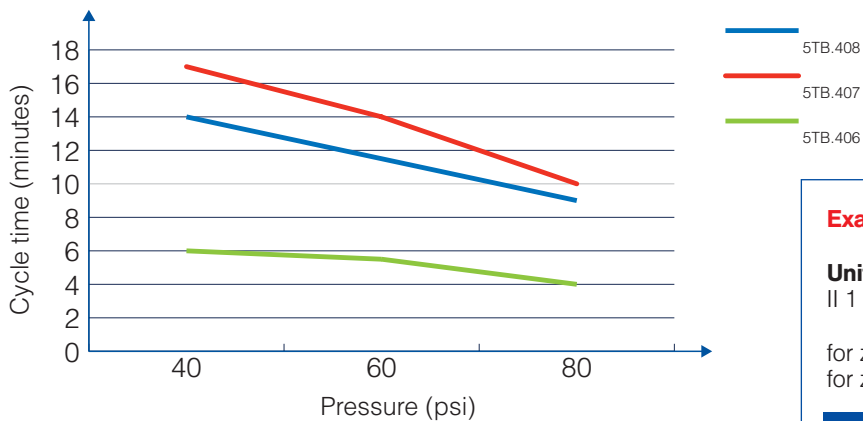
Cycle time depending on pressure of series 5TB
