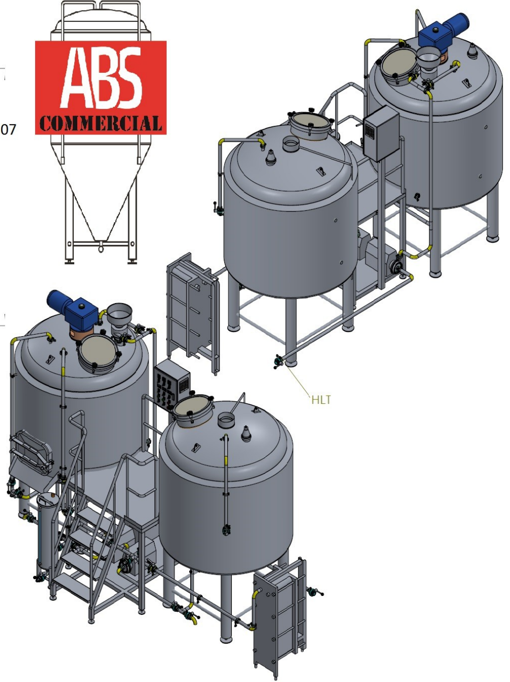
ABS-COMMERCIAL 15 BARREL BREW HOUSE MODEL: BH15BBL
